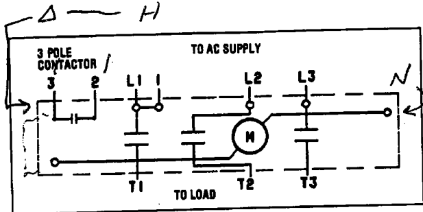
Fig. 5 Connection Diagram A201
