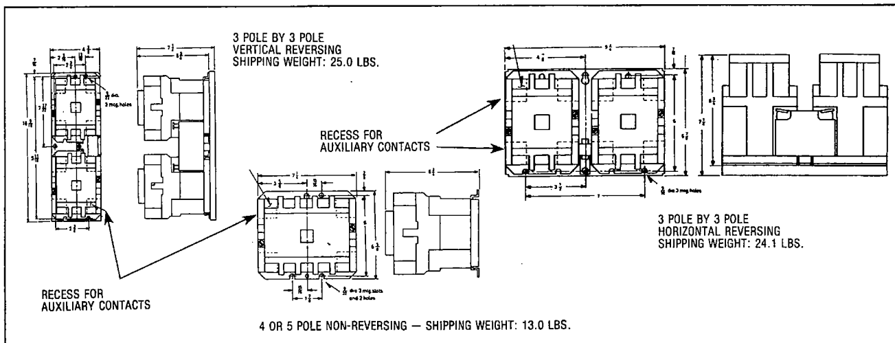
Fig. 3 Dimension Drawings (Dim. in inches)
