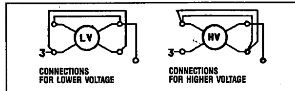
Fig. 4 Dual Voltage Coil Connections
