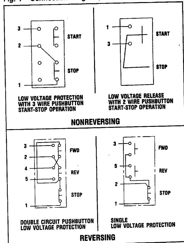
Fig. 8 Control Station Connection Diagrams
