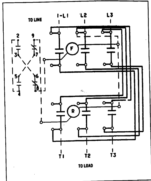
Fig. 7 Connection Diagram, A251
