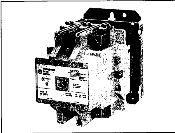
Fig. 1 Size 3, A201 Nonreversing Contactor
