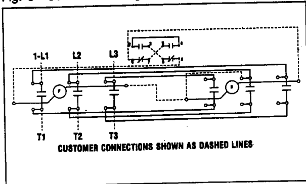
Fig. 6 Connection Diagram, A211
